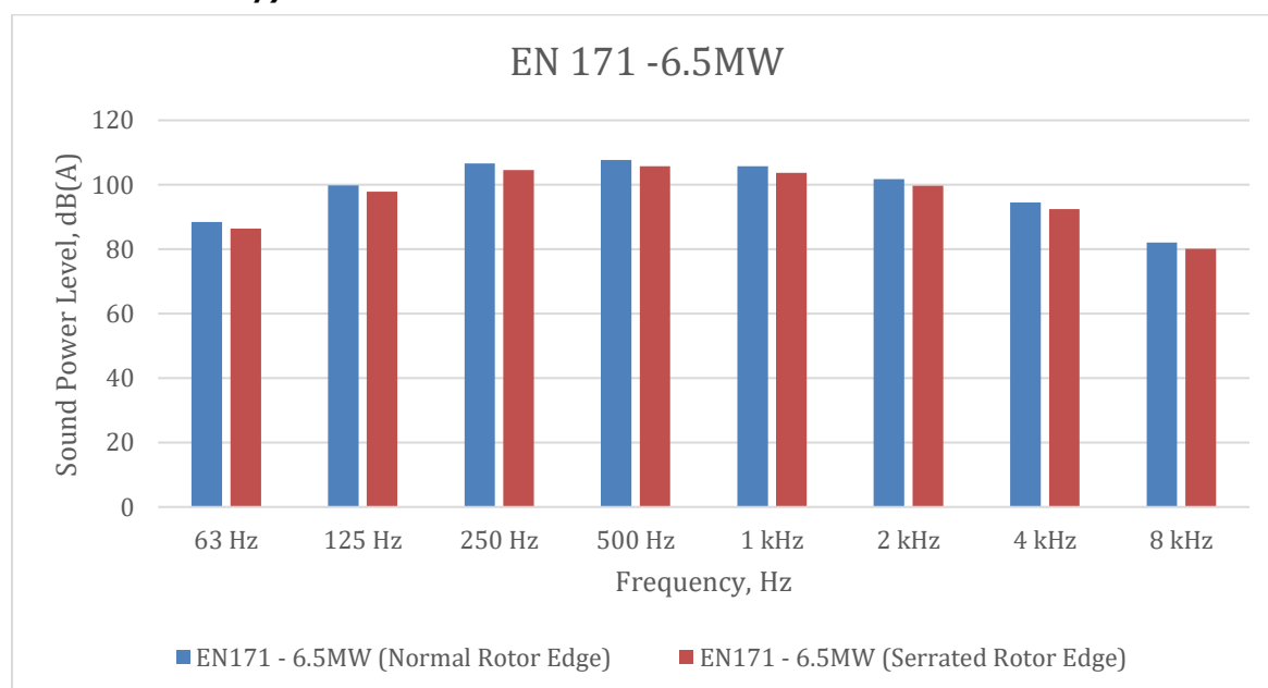
Figure 6-10 Octave Data for the turbines (hub height, 10m/s, not adjusted for uncertainty)
