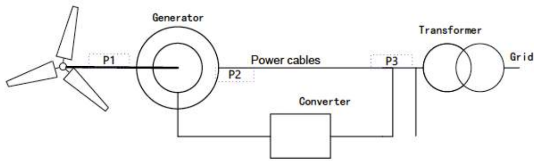
Figure 2-13 Schematic of the Electrical System – Electrical Drive Chain for DFAG
