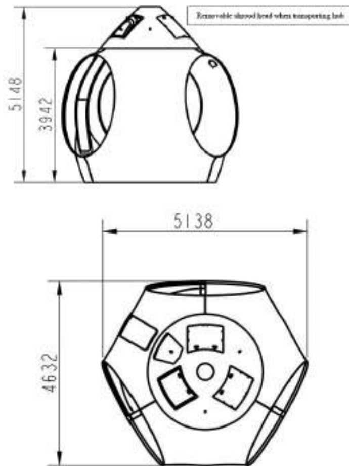
Figure 2-11 Outline of Hub
