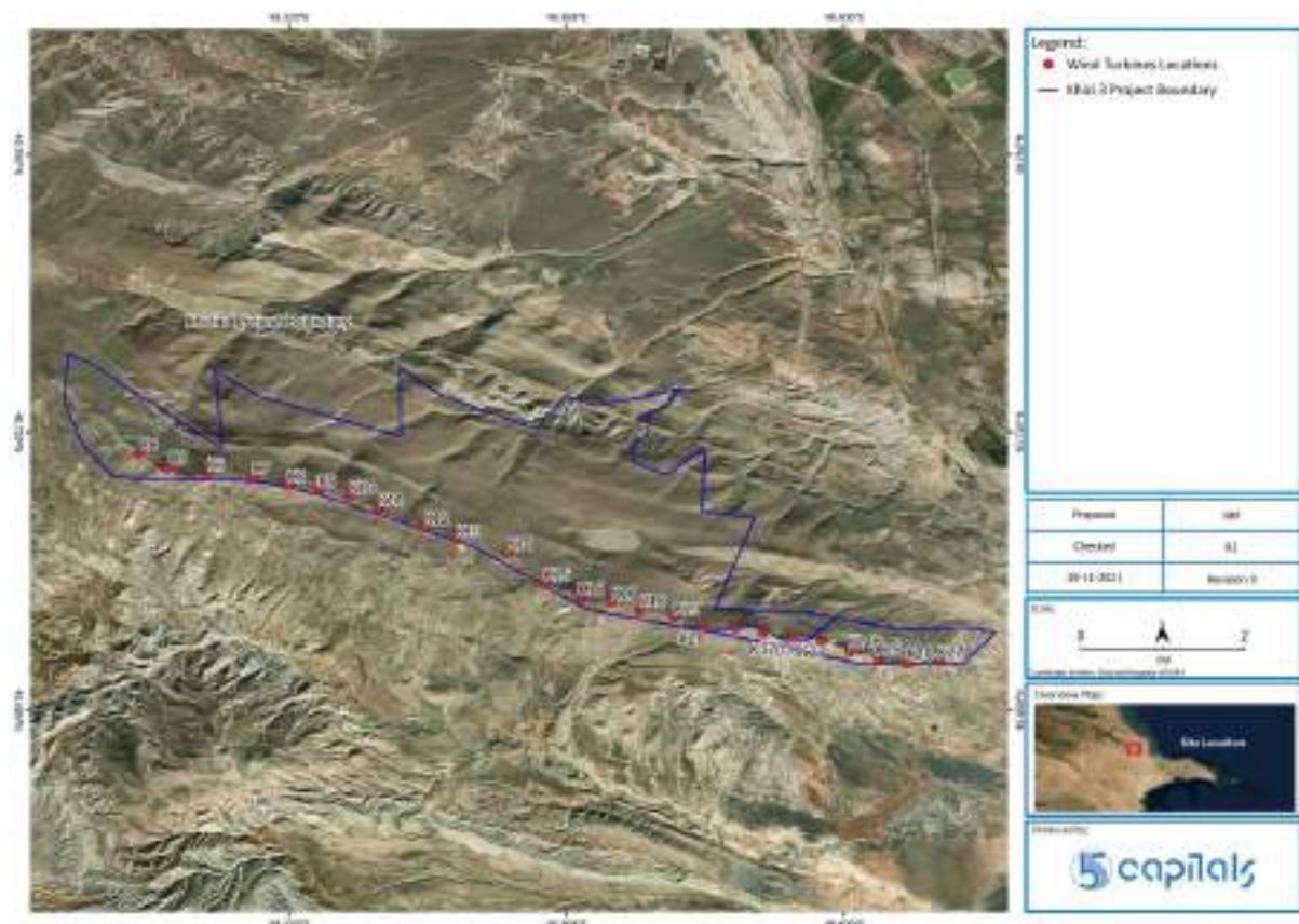
Figure 2-10 Project Layout
