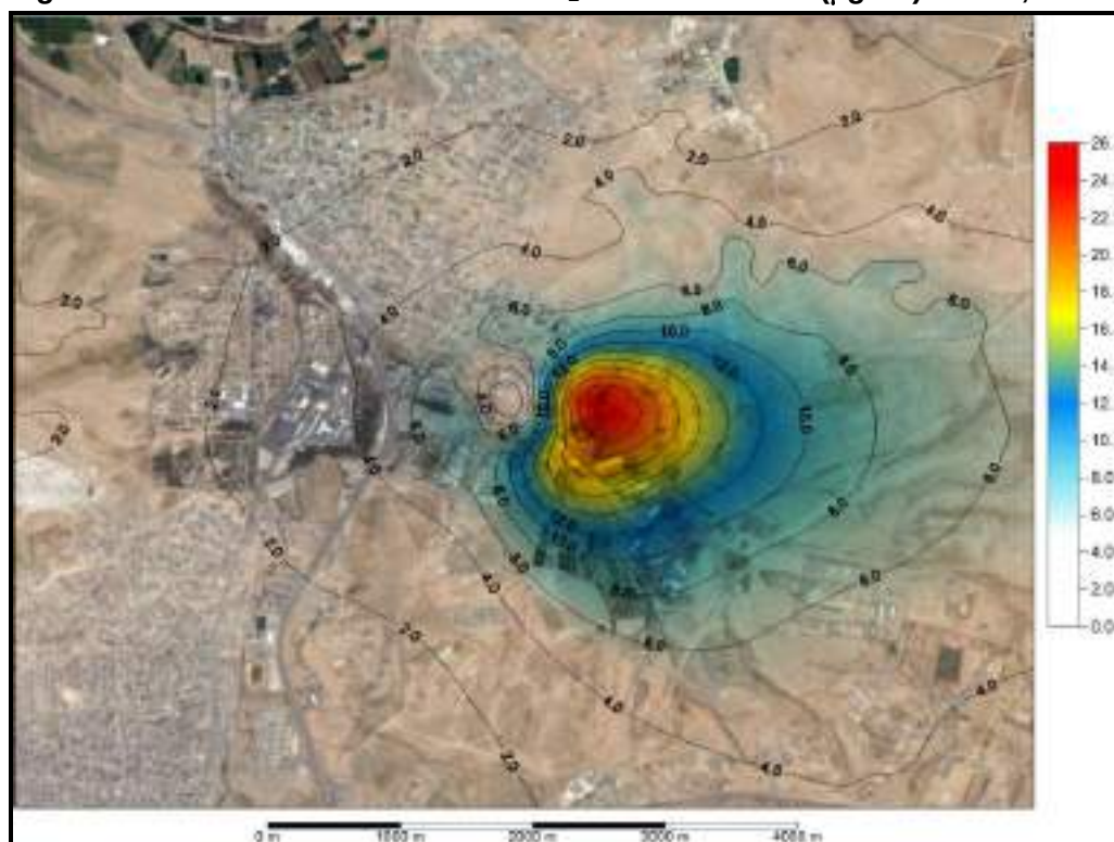
Figure 6.4: Predicted Annual Mean \text{SO}_2 Concentrations ( \mu\text{g}/\text{m}^3 ) – LDO, Combined Cycle
