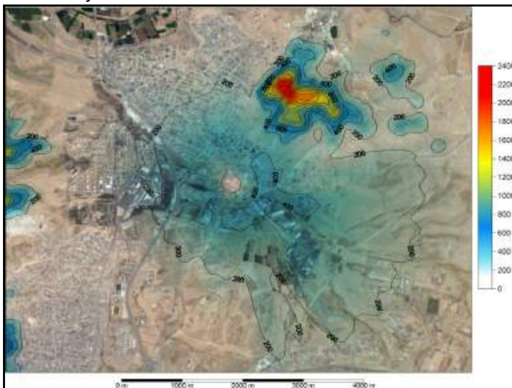
Figure 6.7: Predicted Maximum 10-Minute Mean SO 2 Concentrations ( \mu\text{g}/\text{m}^3 ) – LDO, Combined Cycle
