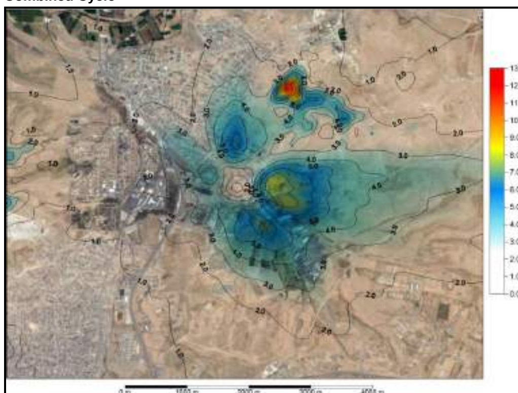
Figure 6.2: Predicted Maximum 24-Hour Mean NO 2 Concentrations (µg/m 3 ) – LDO, Combined Cycle
