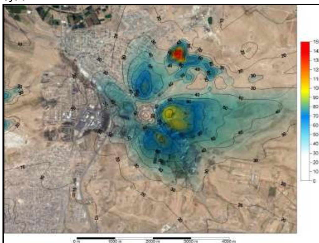
Figure 6.5: Predicted Maximum 24-Hour Mean \text{SO}_2 Concentrations ( \mu\text{g}/\text{m}^3 ) – LDO, Combined Cycle
