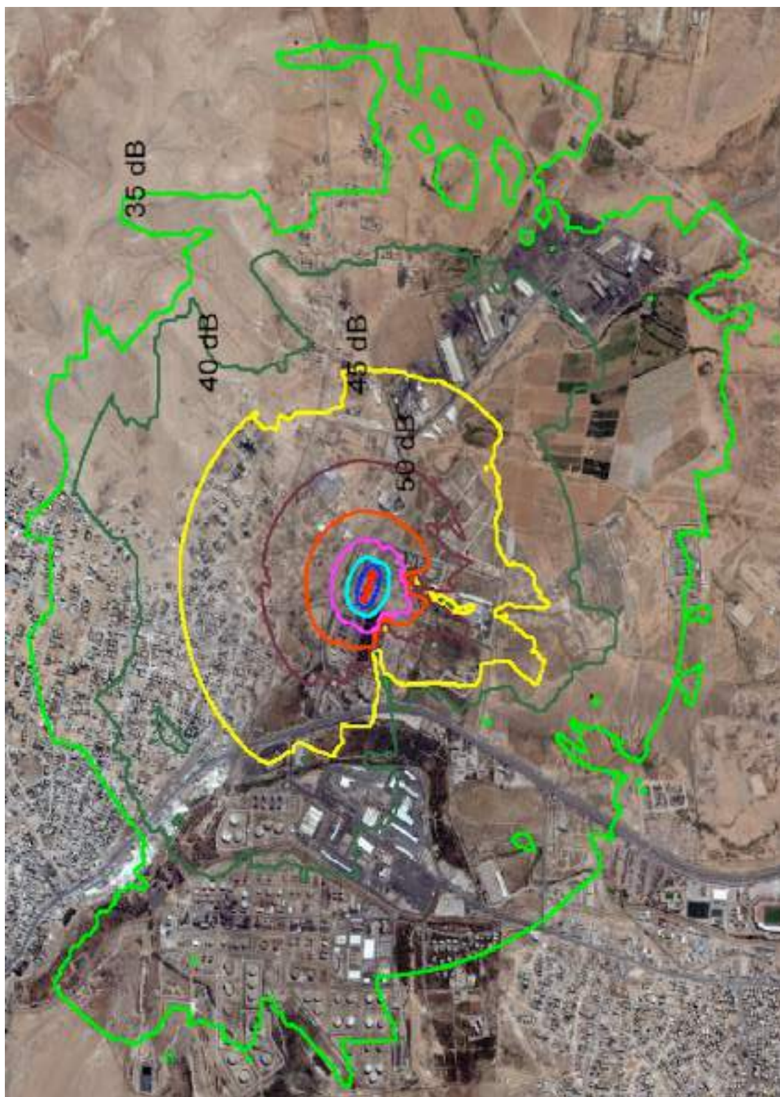
Figure 3 Computed Noise Contours
