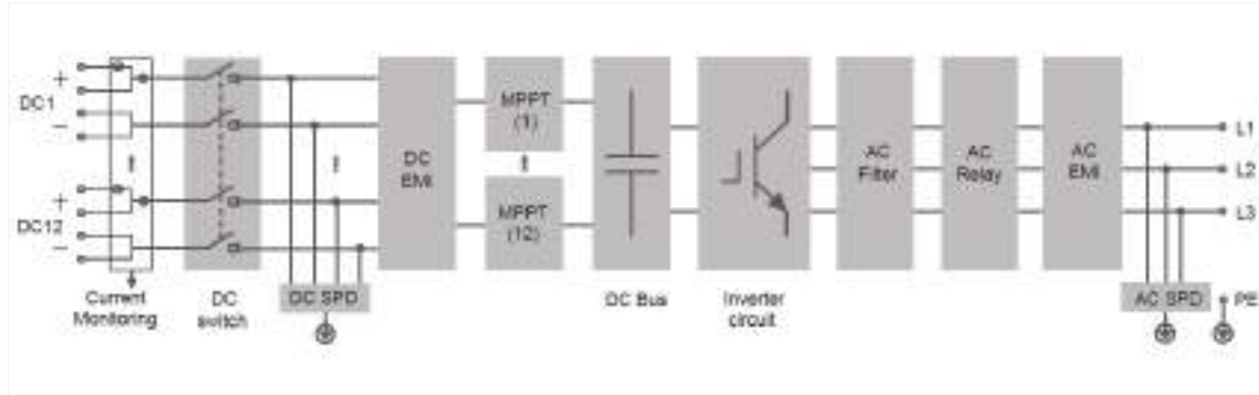
Figure 8 : Principle of electric circuit of an inverter
