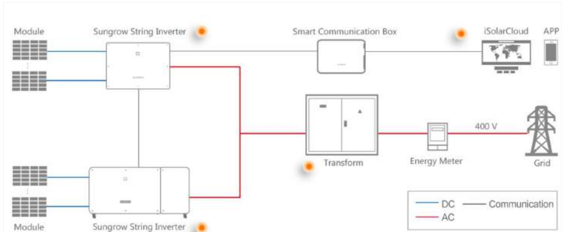
Figure 3 : A model of the Solar Power Plant connection with Al Mowyah electricity Networks
