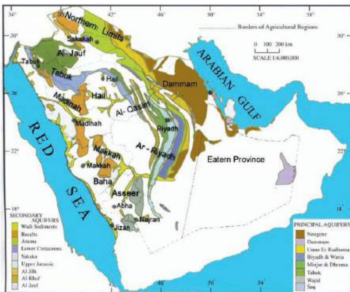
Figure 38: The extension of the outcrop areas of principle and secondary aquifers
