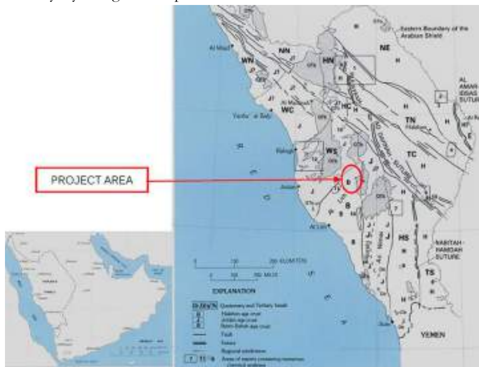
Figure 28 : Project site geology- general overview
