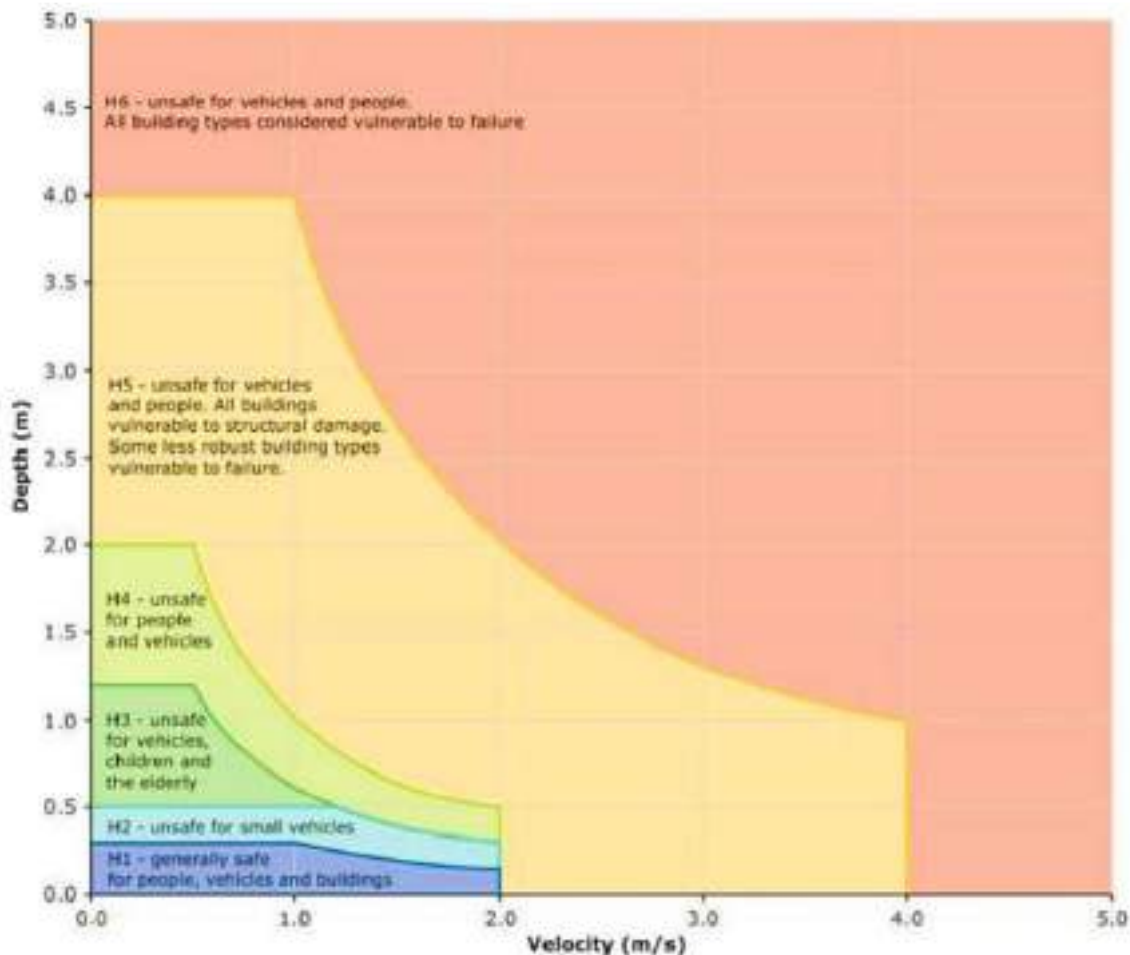
Figure 36: Combined Hazard Curves-Vulnerability Thresholds Classification Limits, Australian Disaster Resilience Handbook
