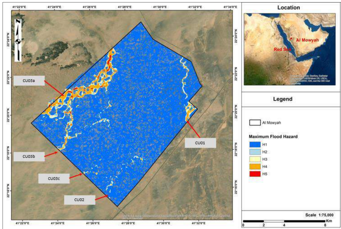
Figure 37 : Classification Flood Hazard (DxV) for the T_r = 100 years.
