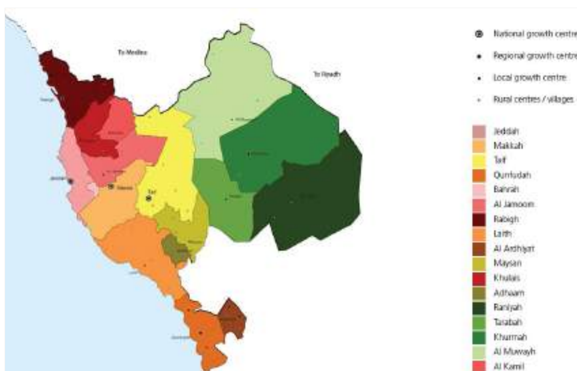
Figure 46 : Administrative boundaries
