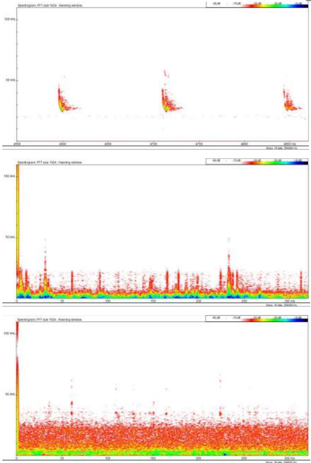
Fig. 3. Degradation of the detector № 6 during its operation at the meteorological masts. Examples of spectrograms of audio files (threshold all files = 10; top down): 01 May 2021 (with bat calls), 01 June 2021, 19 June 2021.
