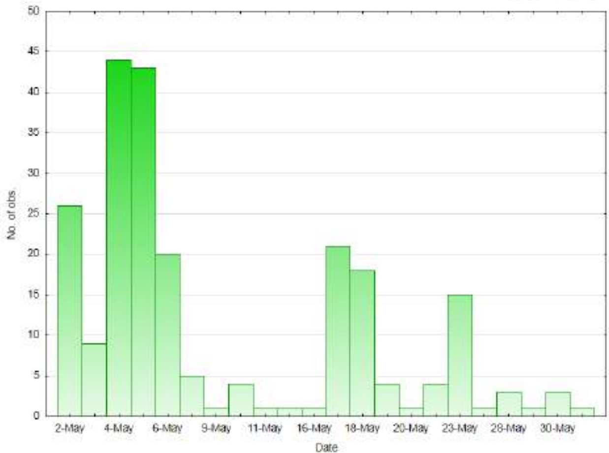
Fig. 4. Bats activity (number of calls for a full night of count) in May (May 2 – June 1) in the vicinity of meteorological mast 8 (MM-8).
