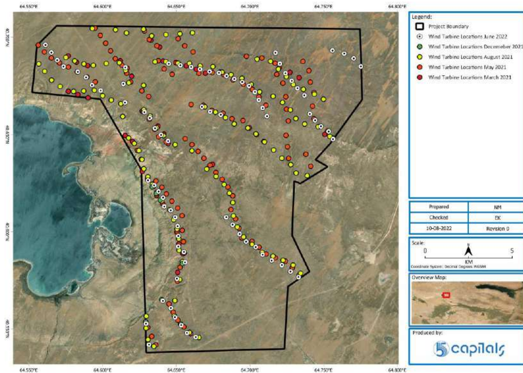
Figure 2-20 Overlay of WTG Considered in March, May, August, November 2021 and June 2022 Showing Difference in WTG Location
