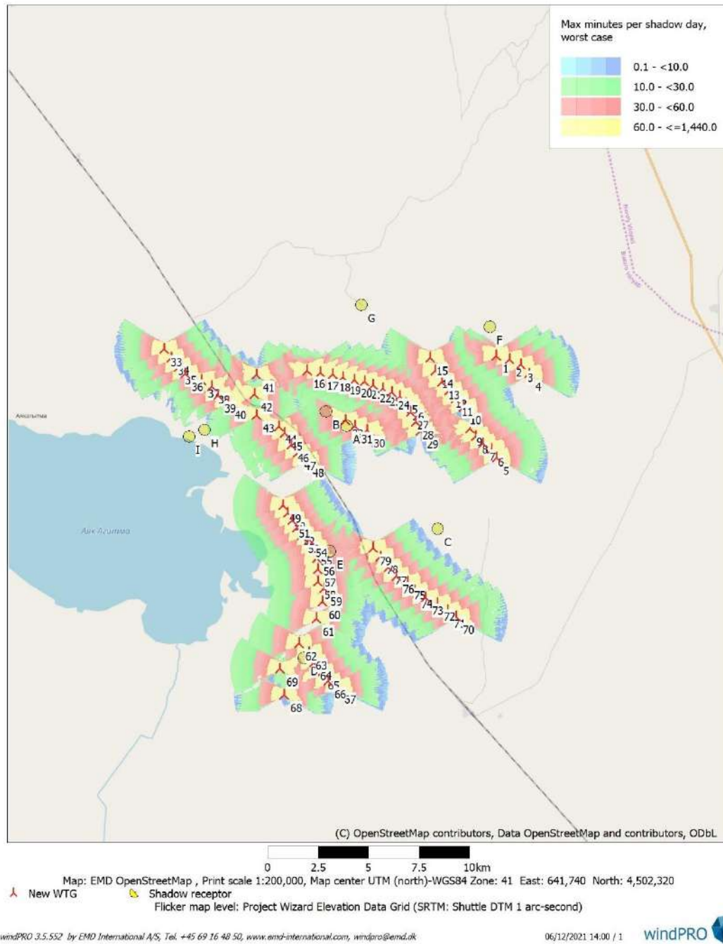
Figure 15-1 WBG/IFC Worst Case Maximum Minutes per Shadow Day
