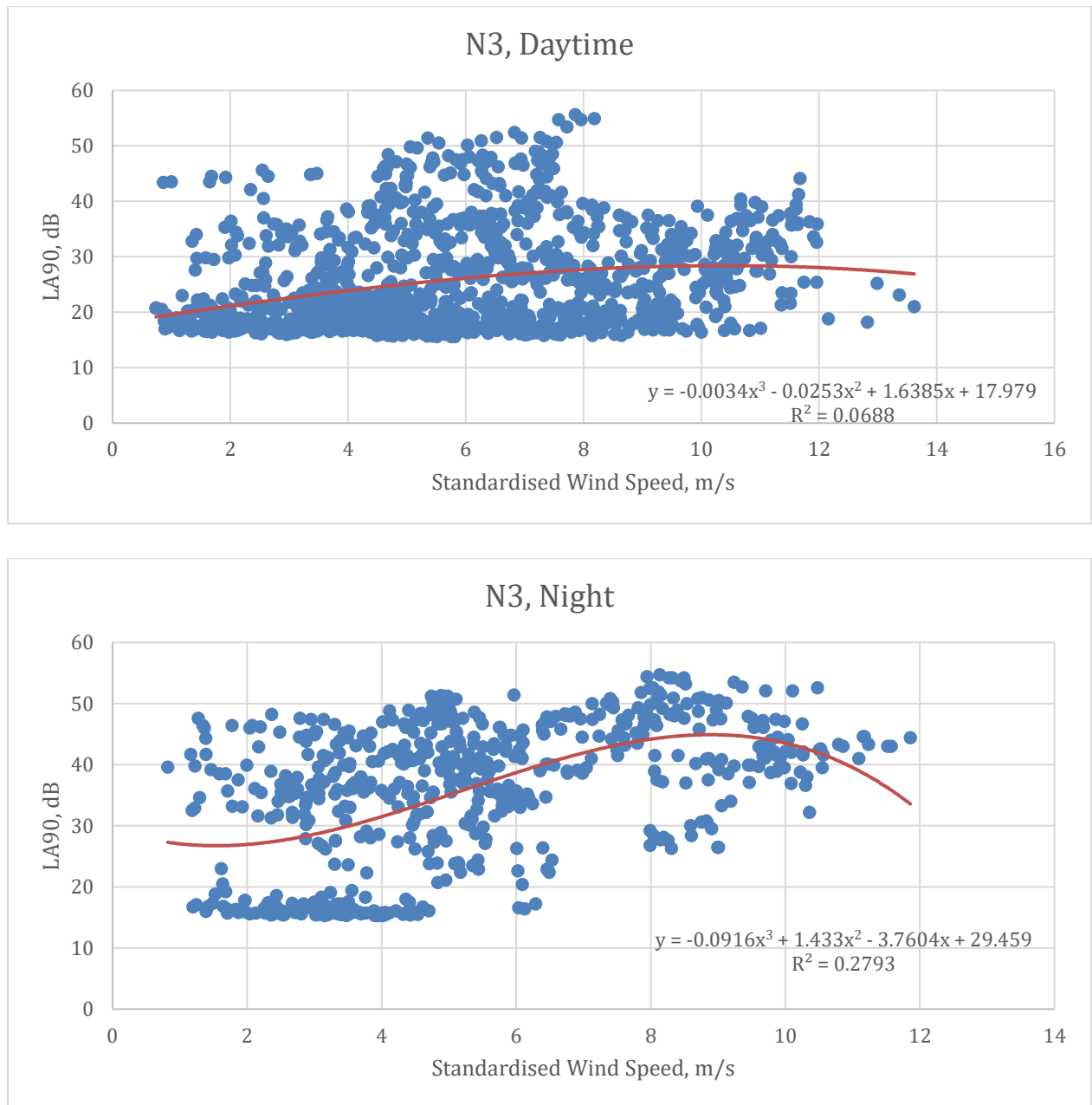
Figure 9-25 Regression Analysis at Survey Location N3
