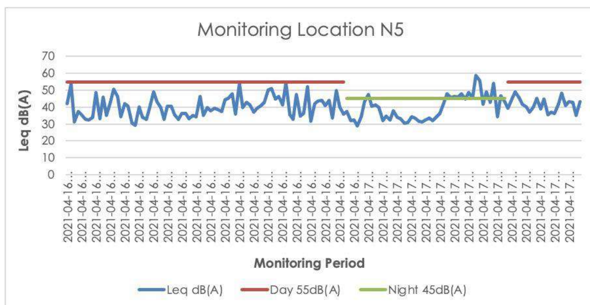
Figure 9-6 Noise Monitoring Result at N5
