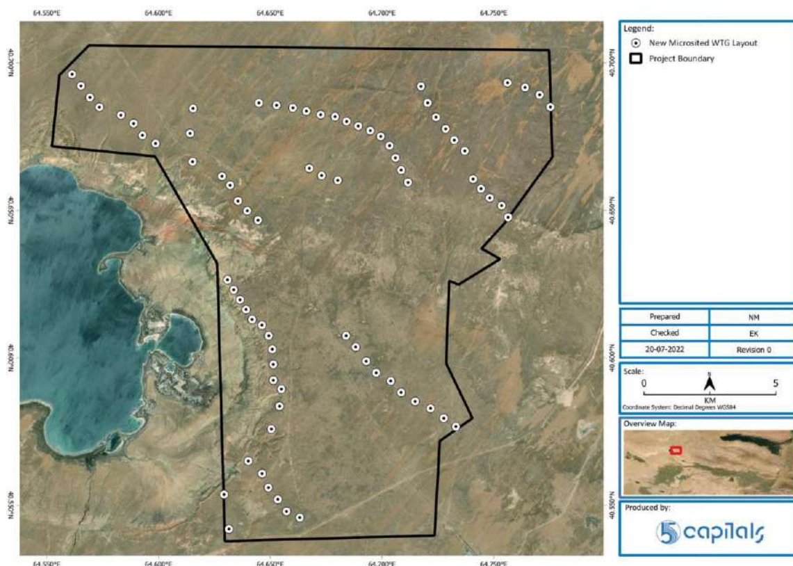
Figure 2-9 Proposed WTG Locations within the Project Site (June, 2022)
