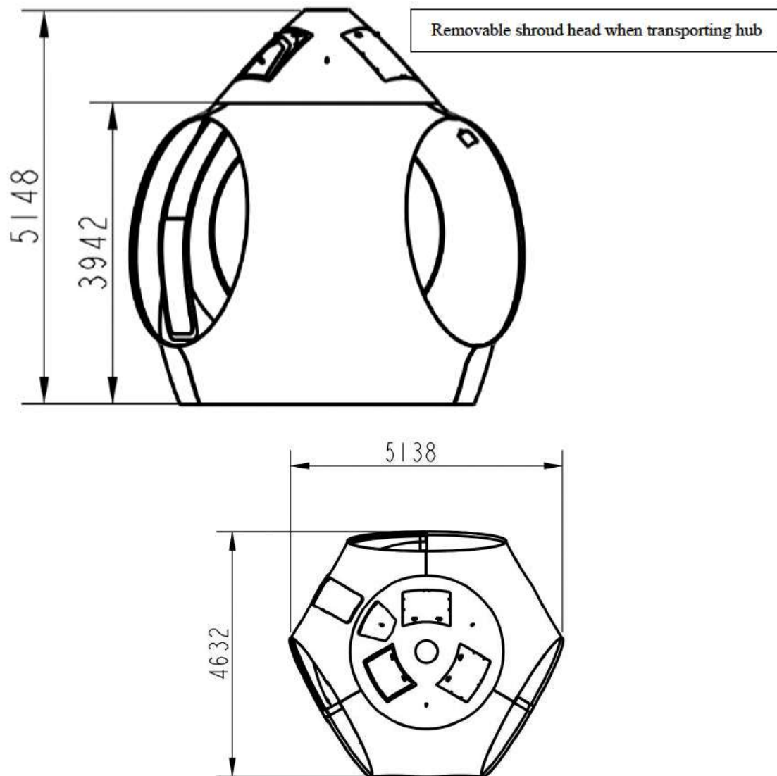
Figure 2-10 Outline of Hub
