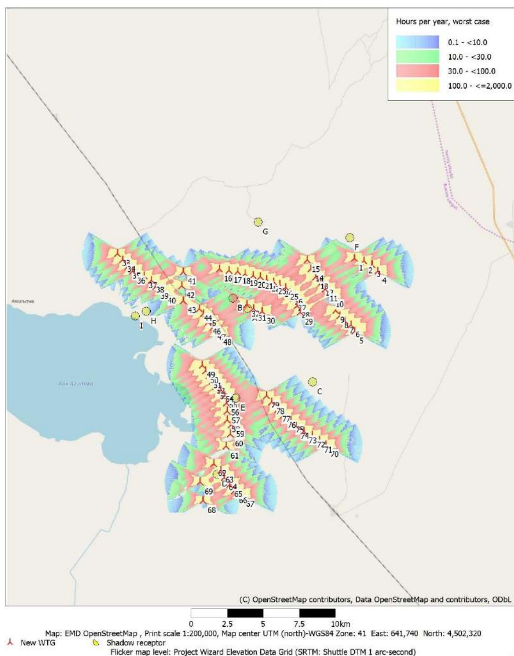
Figure 15-2 WBG/IFC Worst Case Shadow Hours Per Year
