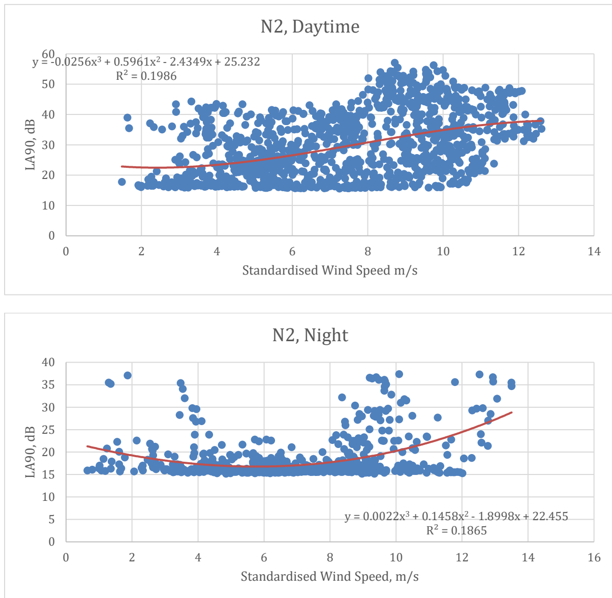
Figure 9-24 Regression Analysis at Survey Location N2
