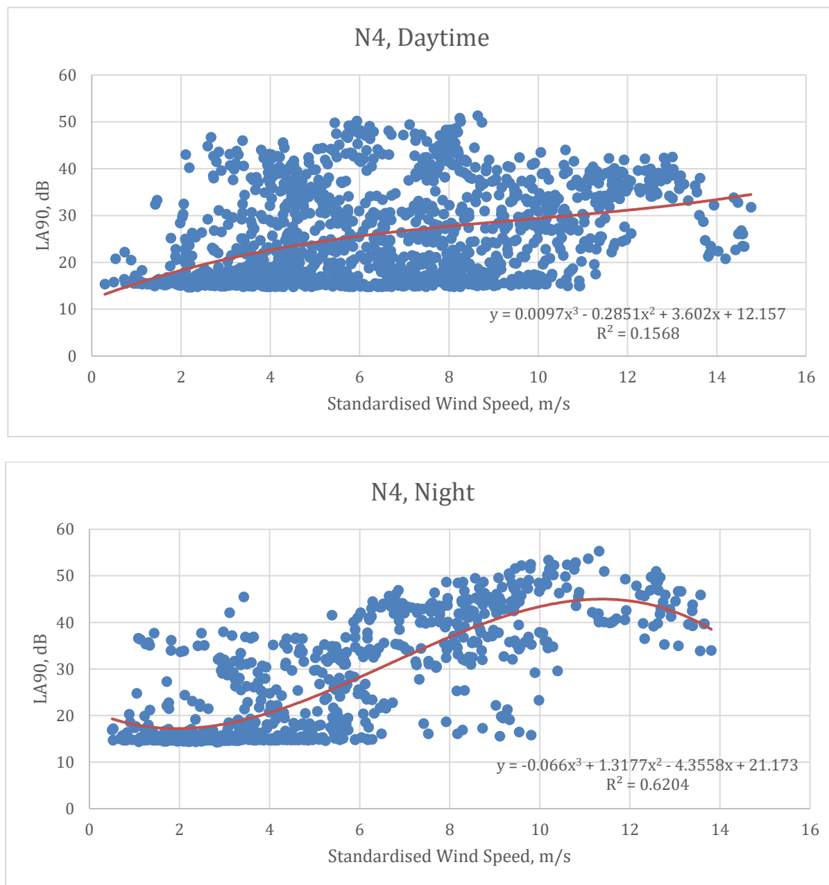
Figure 9-26 Regression Analysis at Survey Location N4
