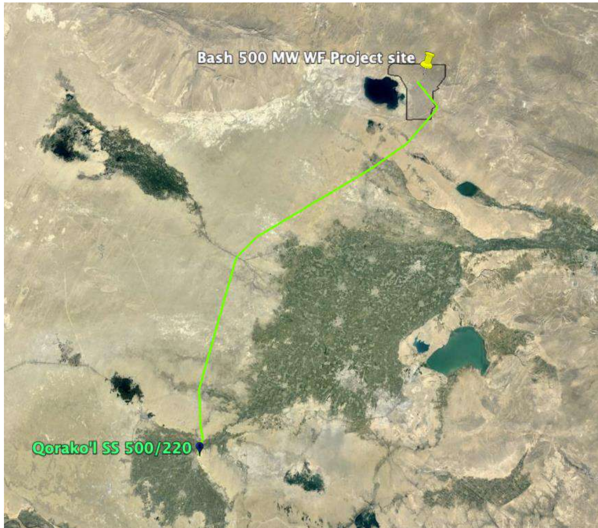
Figure 2-16 Location of 162 km OHTL Route from the Project Site to Kurakul Substation
