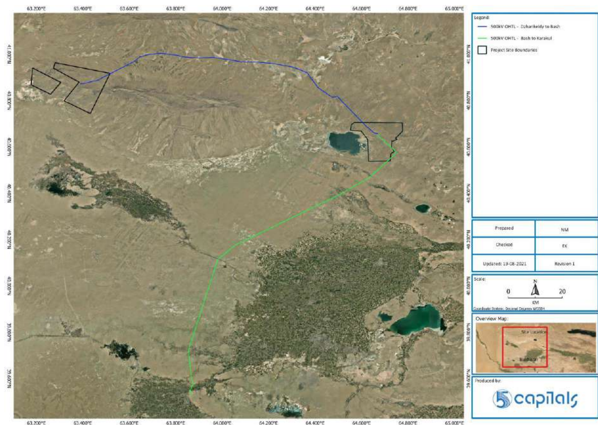
Figure 2-28 Proposed OHTL Alignment – August 2021
