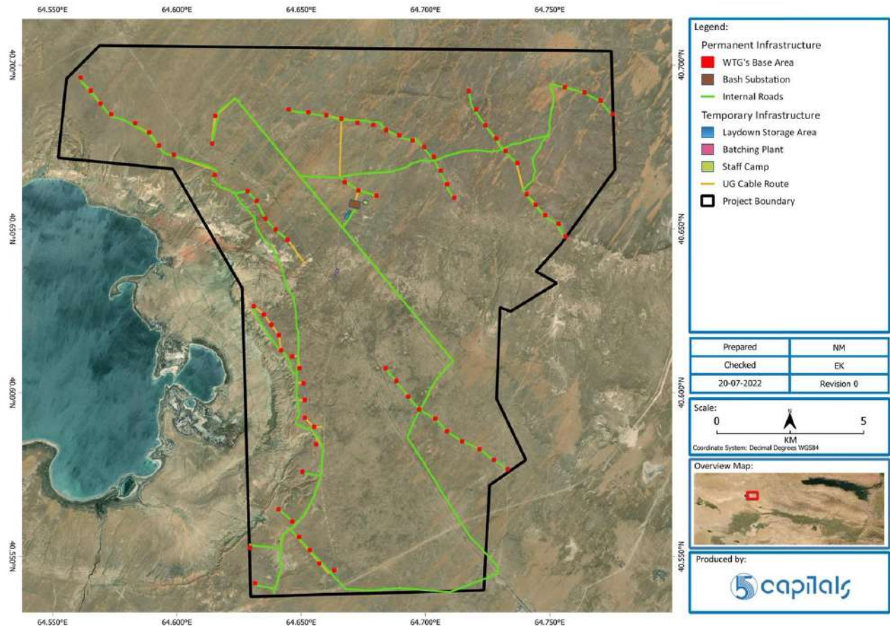
Figure 2-13 Proposed Routing Network of Internal Access Roads (ref. green lines)
